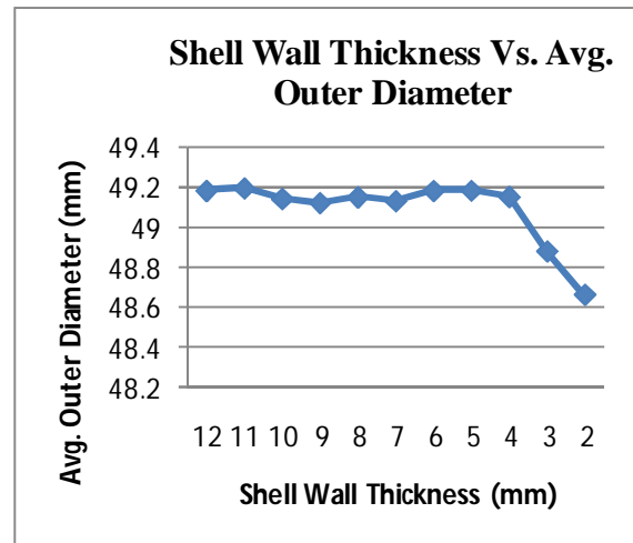
Fig. 5. Effect of Shell Wall Thickness on Outer Diameter for Aluminium Alloy
