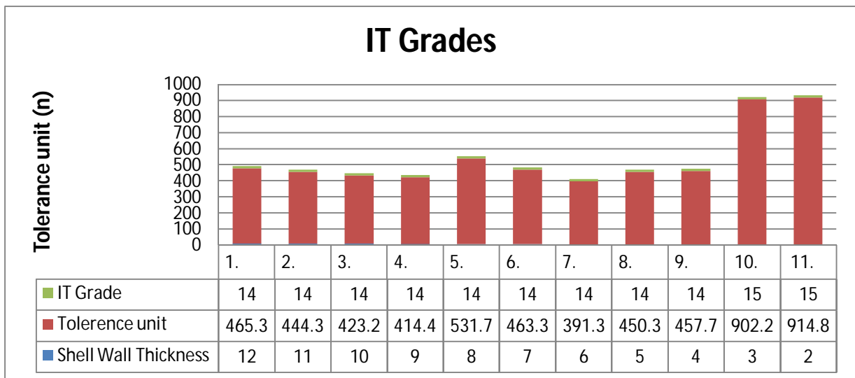
Fig: 20. Effect of Shell Wall Thickness on Tolerance Grade w.r.t. Outer Radius
