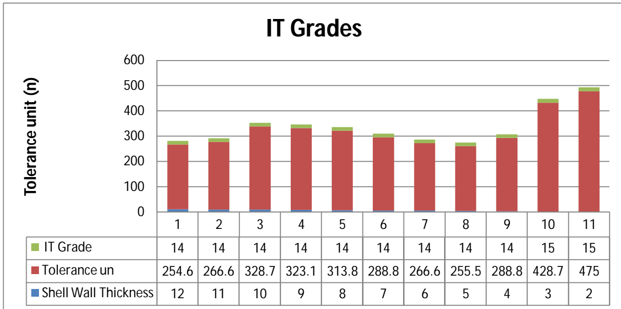
Fig: 17. Effect of Shell Wall Thickness on Tolerance Grade w.r.t Curve Radius
