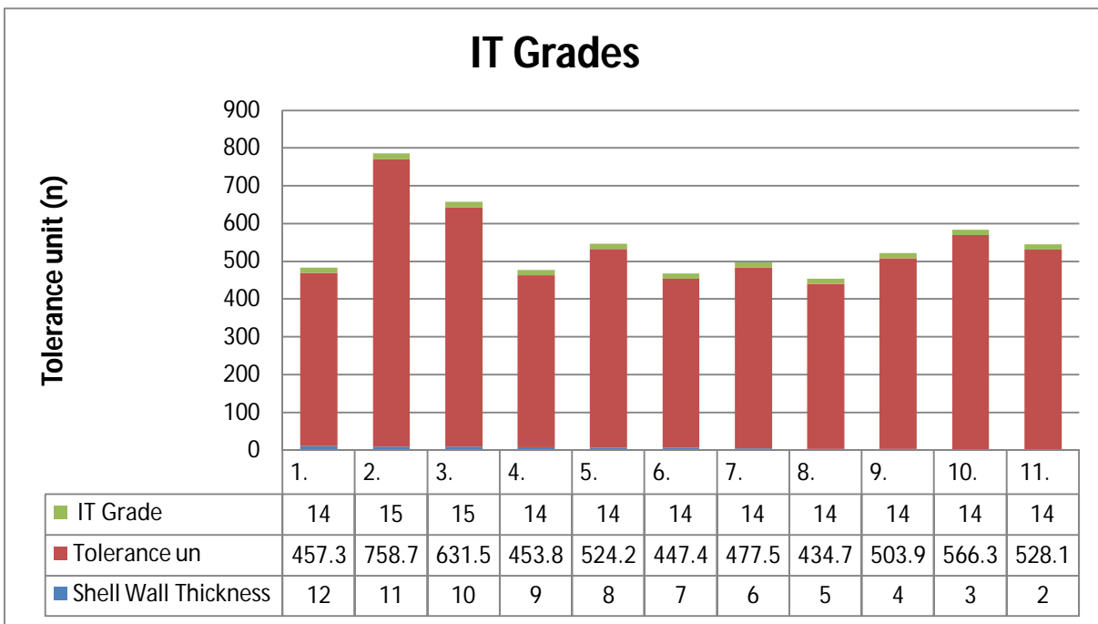
Fig: 18. Effect of Shell Wall Thickness on Tolerance Grade w.r.t. Outer Radius
