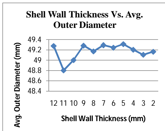
Fig. 8. Effect of Shell Wall Thickness on Outer Diameter for Zinc Alloy
