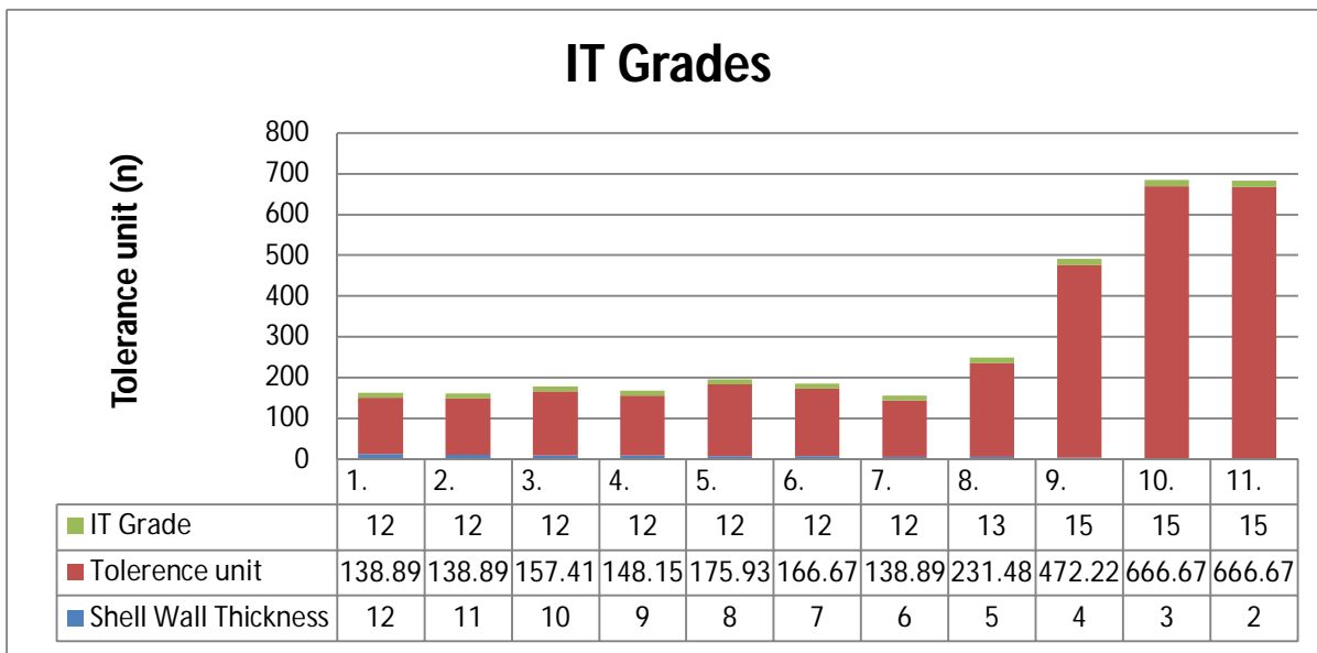
Fig: 21. Effect of Shell Wall Thickness on Tolerance Grade w.r.t Curve Radius
