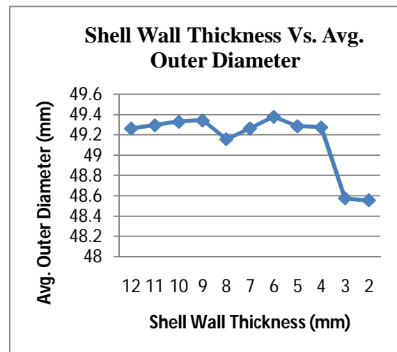
Fig. 11. Effect of Shell Wall Thickness on Outer Diameter for Lead Alloy
