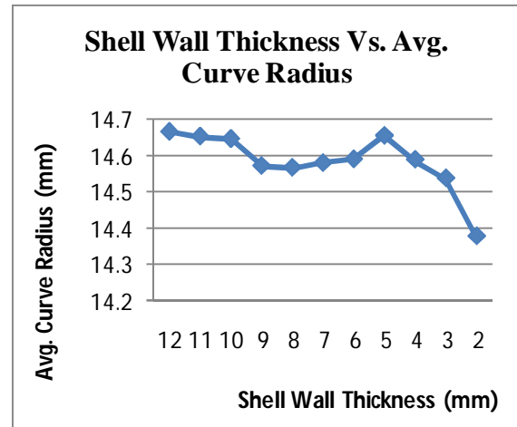
Fig. 9. Effect of Shell Wall Thickness on Curve Radius for Zinc Alloy
