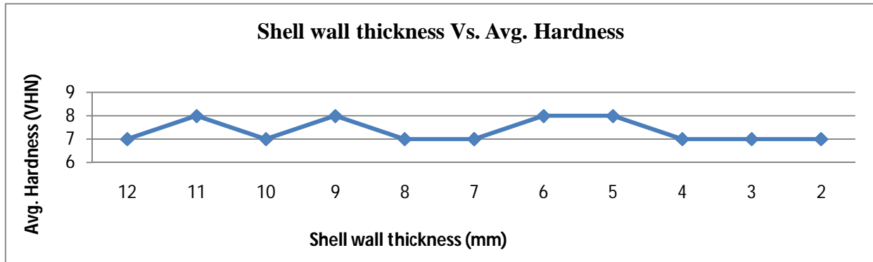
Fig. 13. Effect of Shell Wall Thickness on Surface Hardness for Lead Alloy
