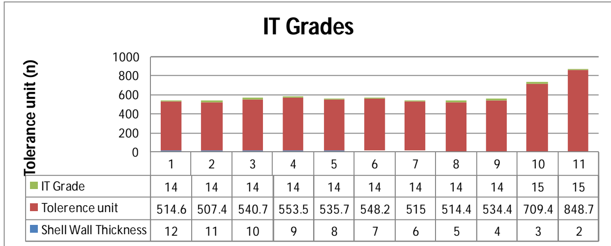
Fig: 16. Effect of Shell Wall Thickness on Tolerance Grade W.R.T. Outer Diameter
