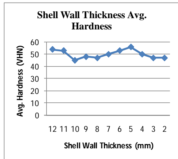
Fig. 10. Effect of Shell Wall Thickness on Surface Hardness for Zinc Alloy
