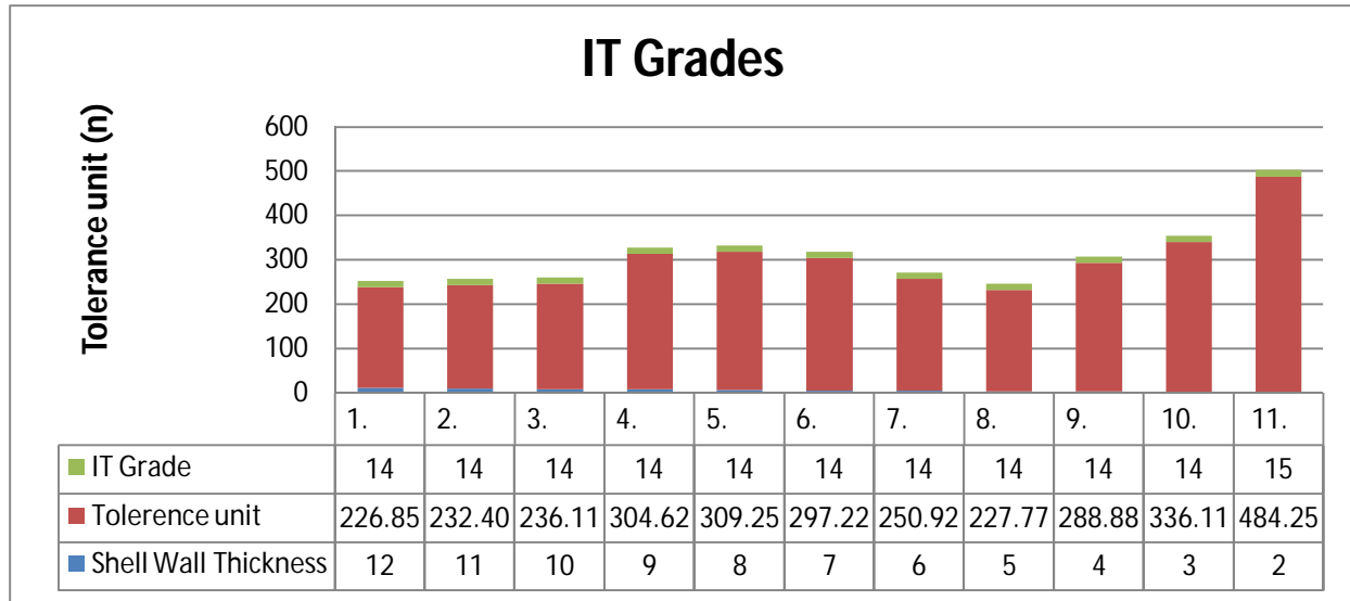
Fig: 19. Effect of Shell Wall Thickness on Tolerance Grade w.r.t Curve Radius
