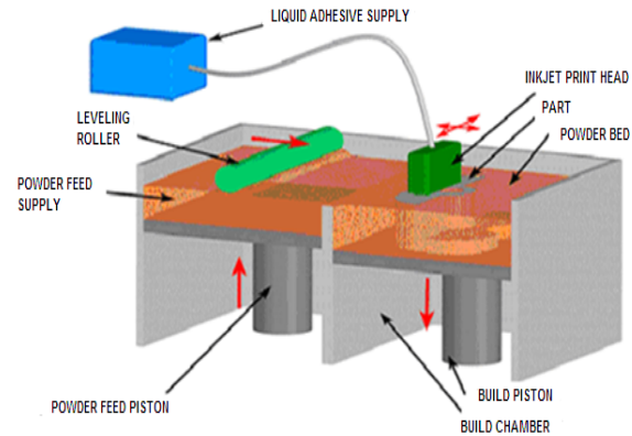
Fig. 1. Three Dimensional Printing (3DP) Processes
