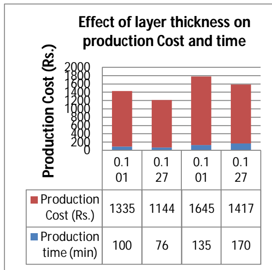
Fig. 4. Effect of Layer Thickness, Part Orientation on Production Cost and Time
