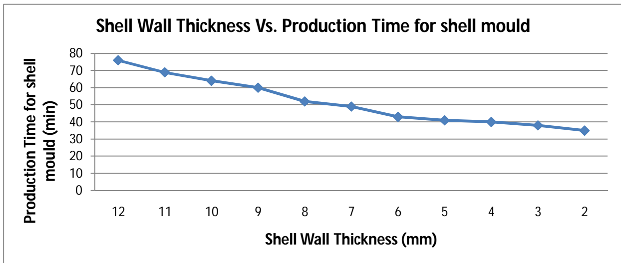
Fig. 15. Effect of Shell Wall Thickness on Production Time for Shell Mould
