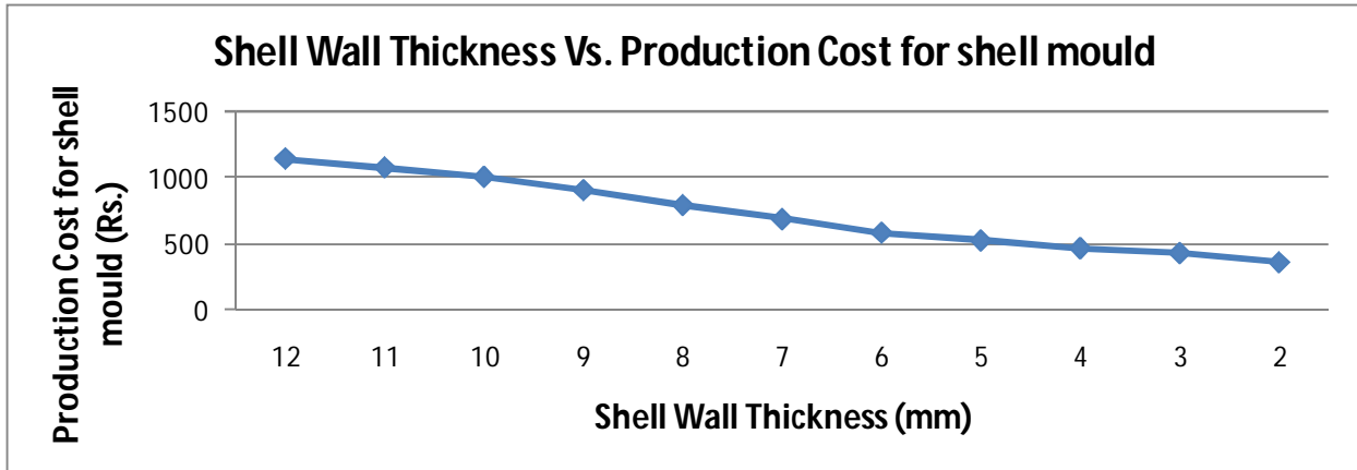
Fig. 14. Effect of Shell Wall Thickness on Production Cost for Shell Mould
