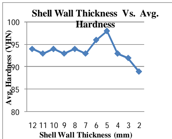
Fig. 7. Effect of Shell Wall Thickness on Surface Hardness for Aluminium Alloy
