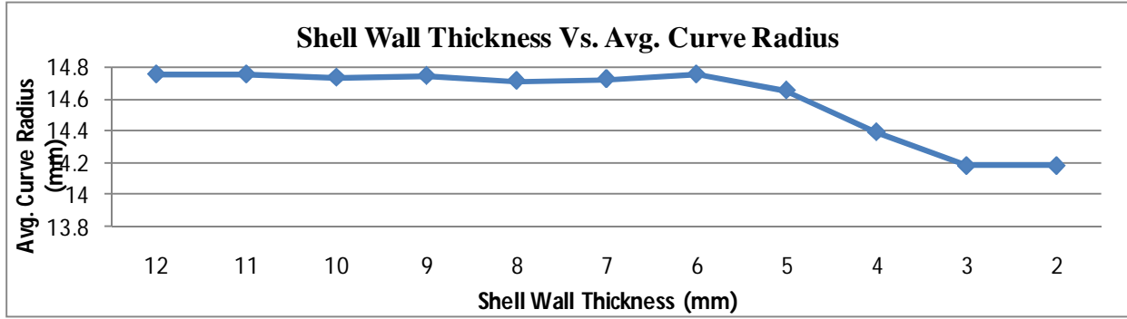
Fig. 12. Effect of Shell Wall Thickness on Curve Radius for Lead Alloy
