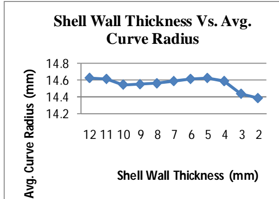
Fig. 6. Effect of Shell Wall Thickness on Curve radius for aluminium alloy
