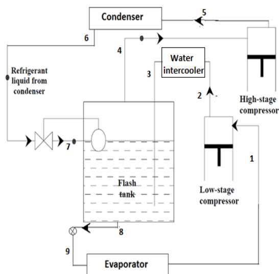
Fig. 1. Schematic Diagram of Two-Stage Vapour Compression Refrigeration System
