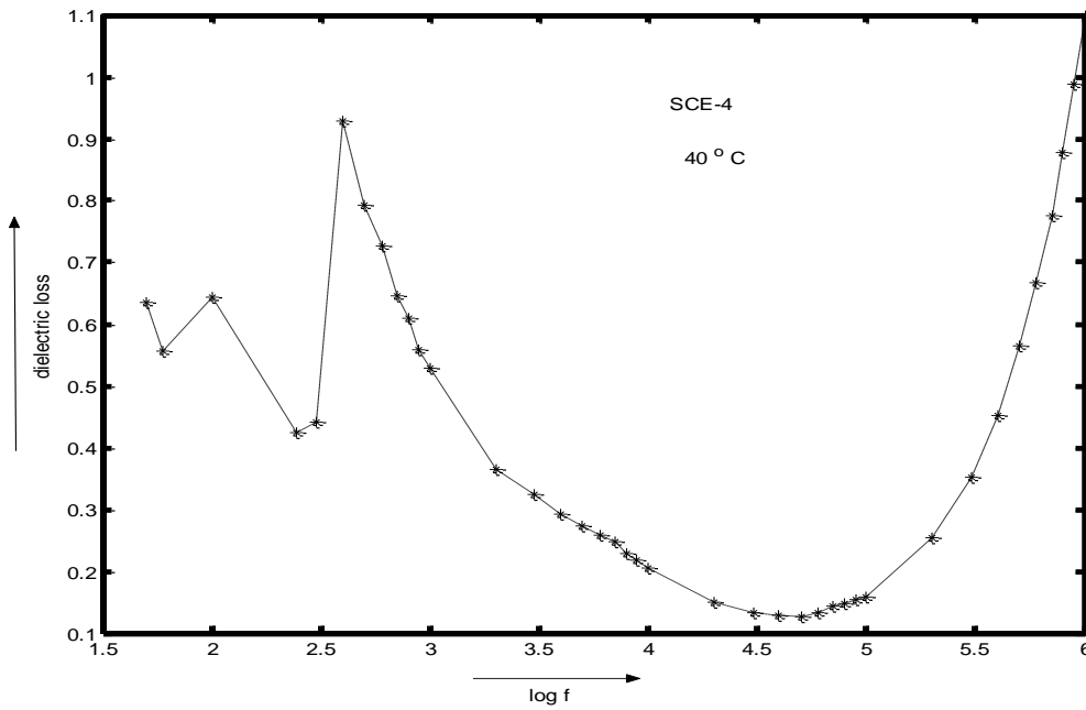
Fig. 2. Dielectric permittivity (imaginary) as a function of frequency
