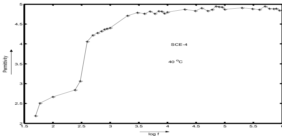
Fig. 1. Dielectric permittivity (real) as a function of frequency
