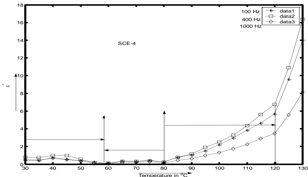
Fig. 4. Temperature dependence of material phases and dielectric absorption
