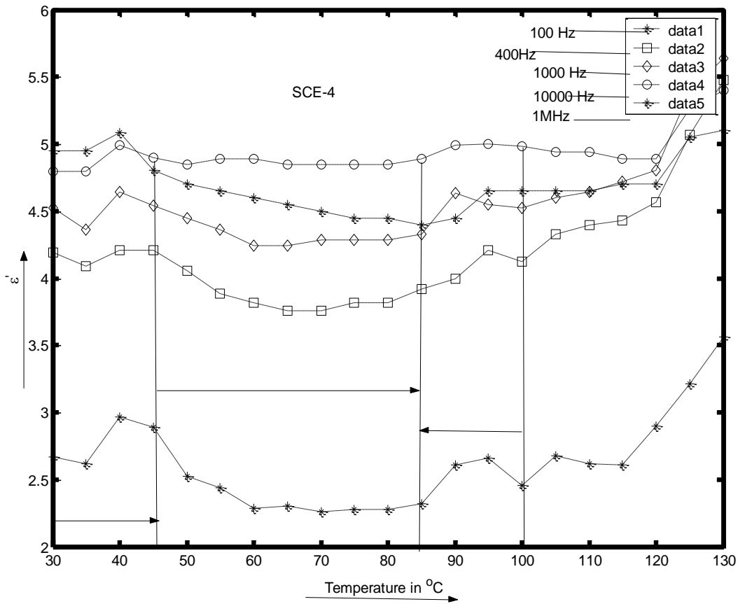
Fig. 3. Temperature Dependence of Dielectric Permittivity
