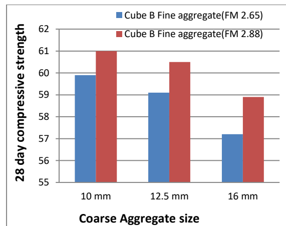
Fig 2: Fig.2 Compressive strength of Cube B for fine aggregate with FM 2.65 and 2.88
