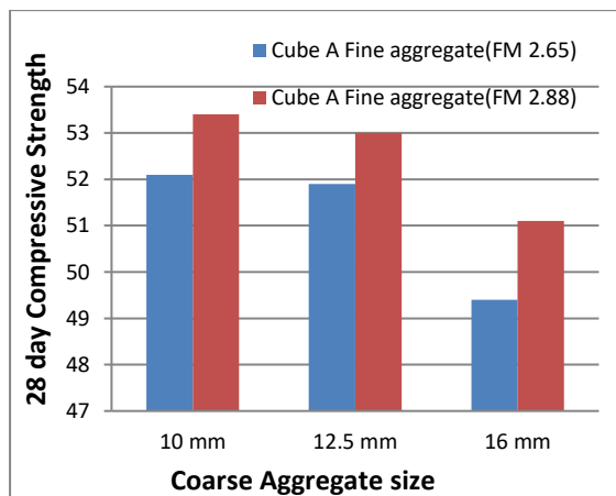
Fig 1: Compressive strength of Cube A for fine aggregate with FM 2.65 and 2.88
