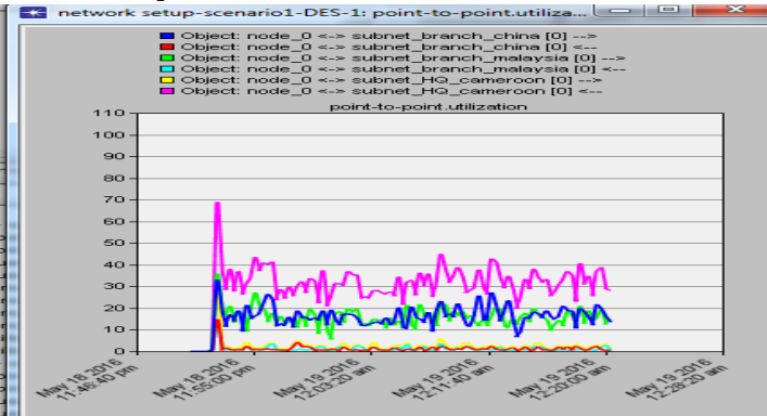
Fig. 16 - Point to point Utilization
