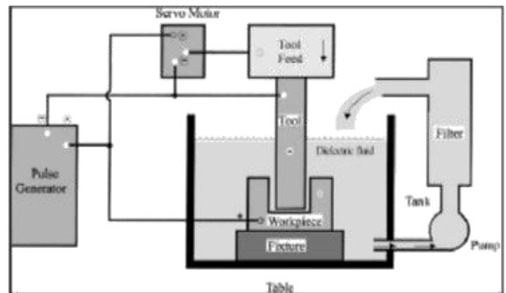
Fig.1: Working principle of EDM[8]
