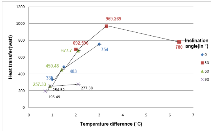
Fig. 5: Variation of heat rejected in condensing section with temperature difference
