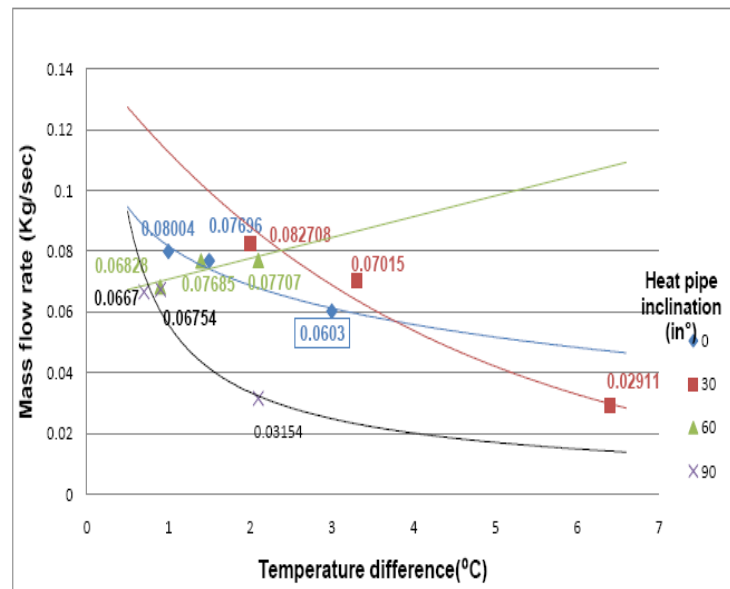
Fig.4: Variation of mass flow rate of external cooling water with temperature difference
