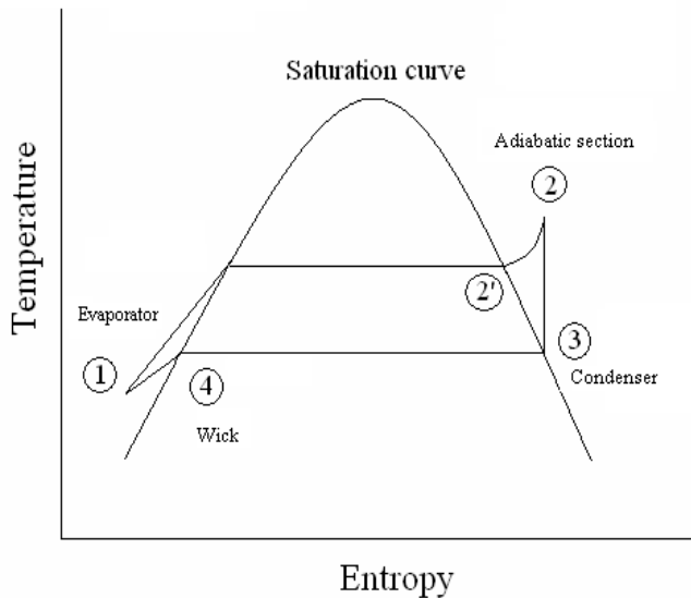
Fig.1: T-S diagram for a heat pipe [21]
