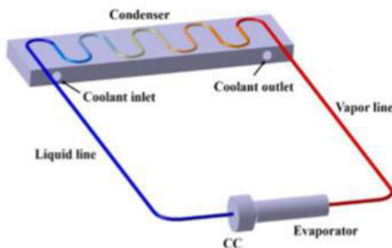
Fig.2: Loop heat pipe system
