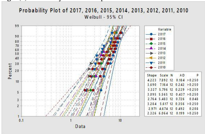
Fig.8 (b) Probability distribution plot for Dibrugarh City
