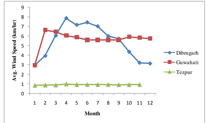
Fig.7 Variation of Avg. Wind Speed with each month from year 2010-2017
