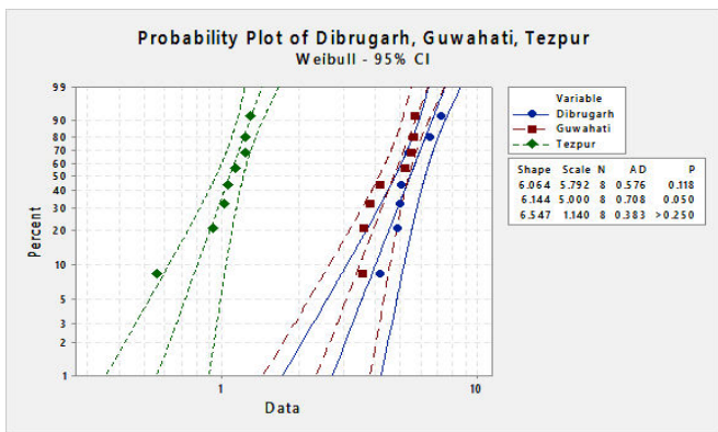
Fig. 8(a) Probability distribution plot for three different cities
