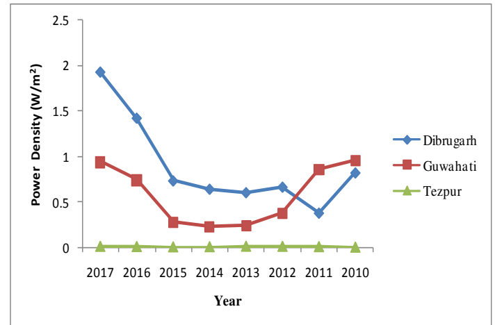
Fig. 9 Variation of Energy Density from year 2010-2017
