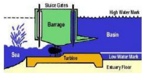
Fig.2: Tidal barrage
