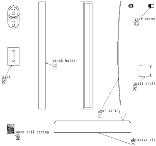
Fig: 6. Different parts of a honing tool
