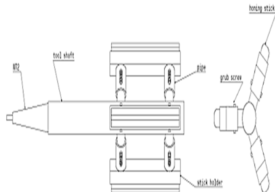
Fig: 5. Honing tool for a drilling machine
