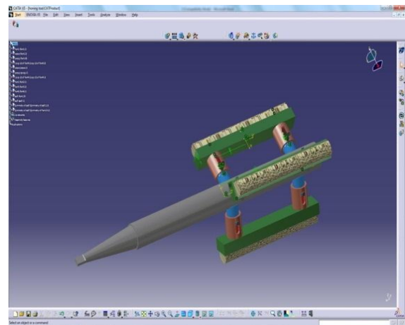
Fig: 3. Designed model of honing tool
