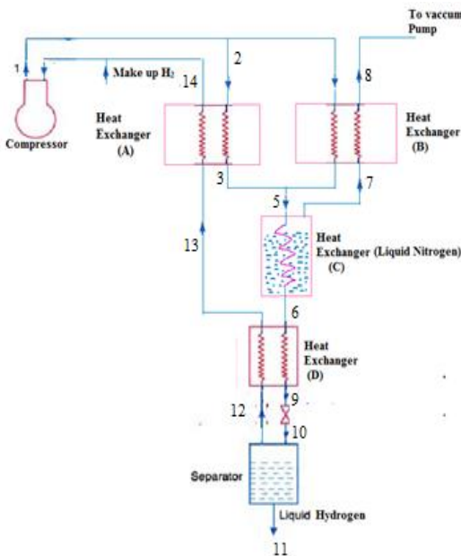
Fig. 1. Block Diagram of Hydrogen Liquefaction System
