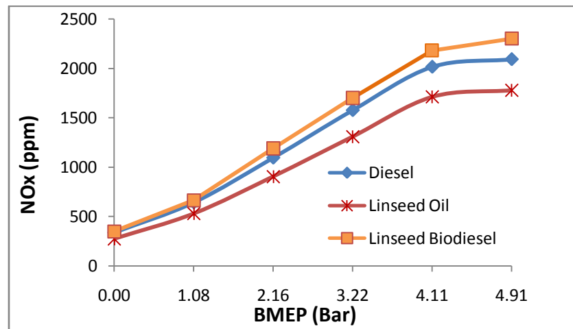
Fig. 6. Variation of oxides of nitrogen with brake mean effective pressure
