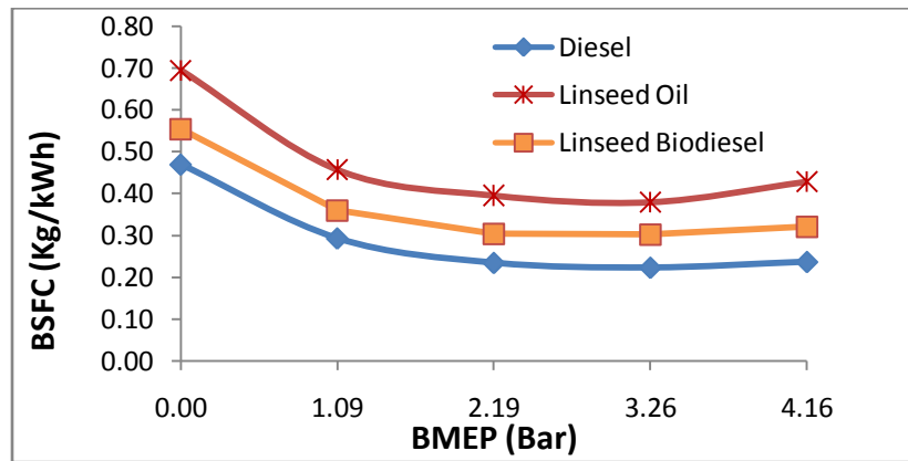
Fig: 5. Variation of brake specific fuel consumption with brake mean effective pressure
