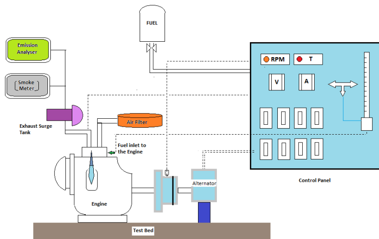
Fig. 3. Schematic diagram of experimental test rig
