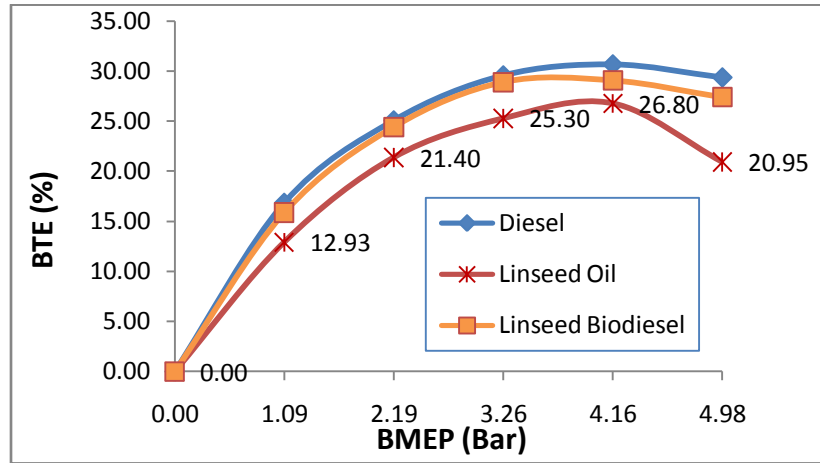
Fig: 4. Variation of brake thermal efficiency with brake mean effective pressure
