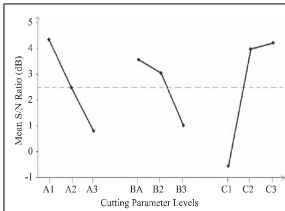
Fig 2: S/n Ratio Graph for Surface Roughness
