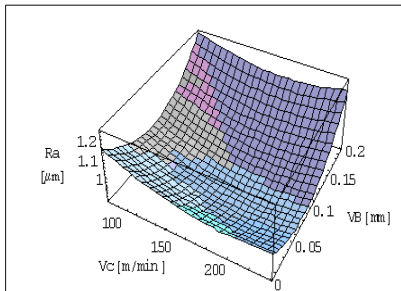
Fig 7: Roughness Surface Variation with Cutting Speed and Flank Wear
