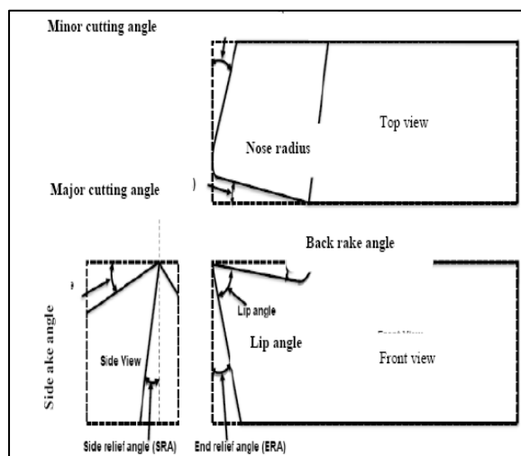
Fig 1: Cutting Tool Nomenclature [Ref 3]
