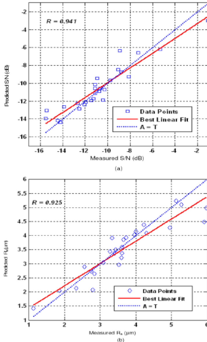
Fig 4: Comparison of Measured and Predicted Values : [Ref 12] (a) for S/N Ratio; (b) for Ra
