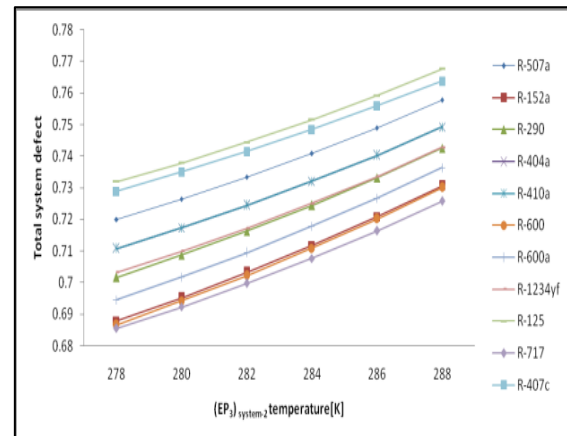
Fig 20: Evaporator-3 Temperature of System-2 Versus Total System Defect
