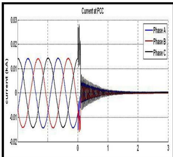
Fig 1: Inverter Currents During a Three-Phase FaultClose to PCC – Model 1 (time in cycles)
