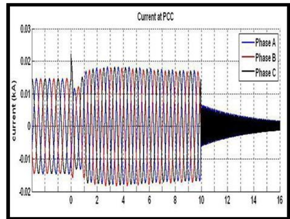
Fig 2: Inverter currents during a three-phase fault close to PCC – Generic Model (time in cycles)
