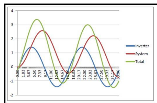
Fig 4: Example of Total Fault Current Comparison (Assuming One Per Unit Rated Inverter Current on System Base)
