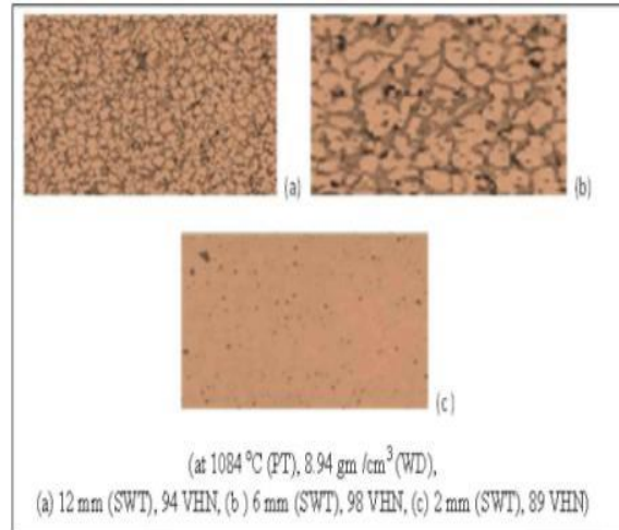
Fig 14: Surface Photomicrograph of Brass Alloy Casting
