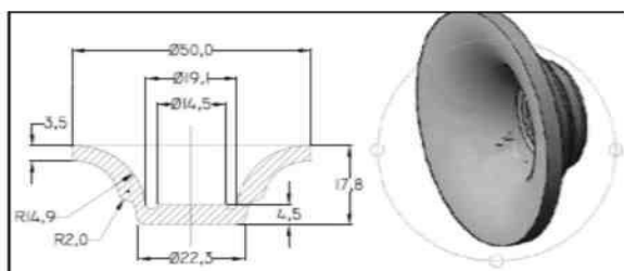
Fig 1: Selected Component with Dimensions
