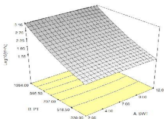
Fig 7: Effects of SWT and PT on Vickers Hardness Number
