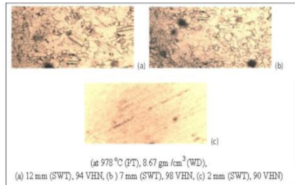
Fig 15: Surface Photomicrograph of Bronze Alloy Casting
