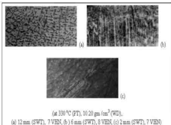
Fig 12: Surface photomicrograph of Pb alloy casting
