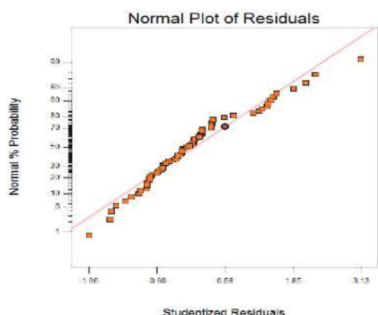
Fig 5: Normal Probability Plot of the Residuals For Hardness
