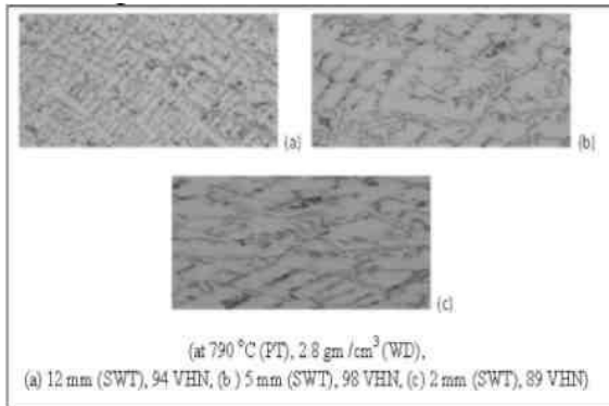
Fig 11: Surface Photomicrograph of Zn Alloy Casting
