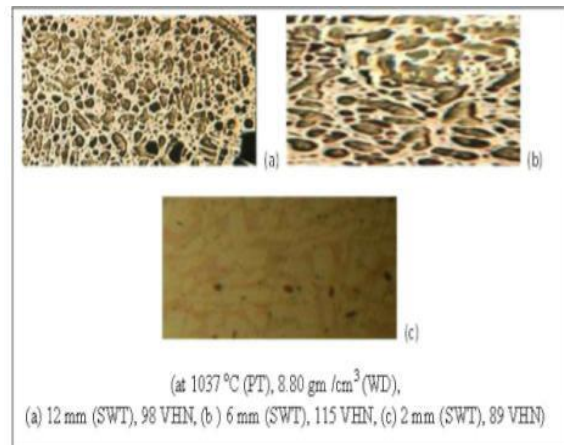
Fig 15: Surface Photomicrograph of Bronze Alloy Casting
