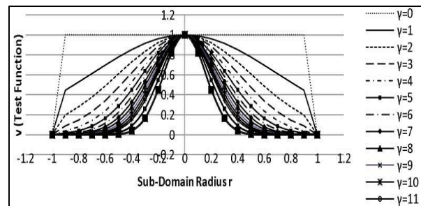
Fig. 2. Variation in Test Function with sub-domain radius r v/s \gamma scaling parameter for exponential test function
