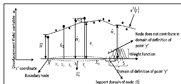
Figure 1- Schematic representation of Error e_i for a field node 'i', support domain of a node 'x', domain of definition of point 'y', weight function for 1-D case of MLSAS in meshless method.
