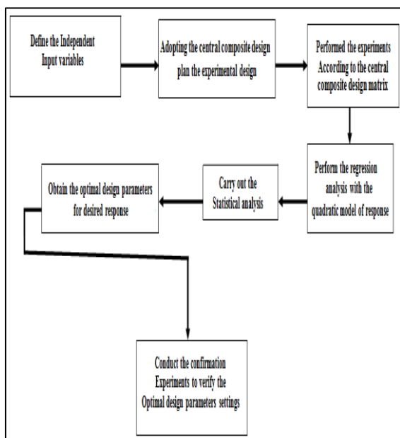
Fig 3: Steps Involved in Central Composite Design [20]
