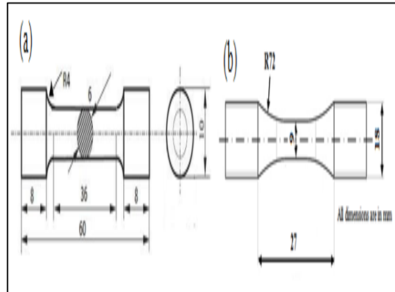
Fig 4: Sample Specification; (a) Tensile Sample, (b) Fatigue Sample [18]
