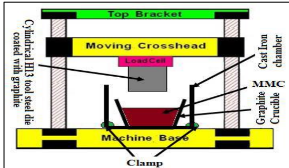
Fig 2: Schematic Diagram of Squeeze Casting Process on UTM
