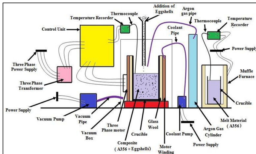
Fig 1: Experimental Set-up of Electromagnetic Stir Casting Process
