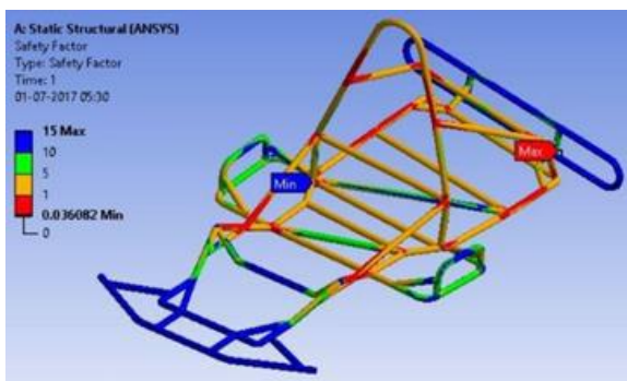
Fig 10 (d): Factor of Safety
