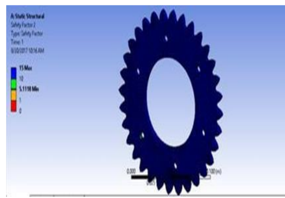
Fig 33 (c): Factor of safety
