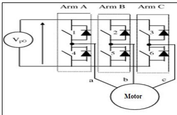
Fig 1: Topology of a Three-Phase Inverter
