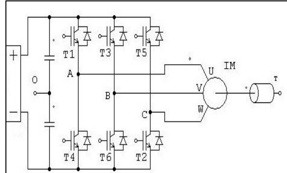
Fig 2: Three Phase PWM Inverter Fed Induction Motor
