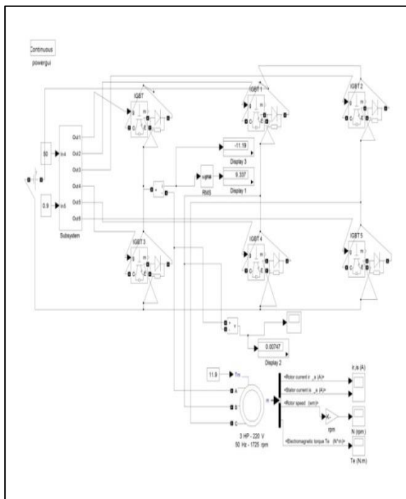
Fig 3: Circuit Diagram of PWM Based VSI Fed Three Phase Induction Motor
