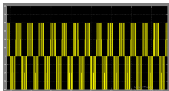
Fig 5: Waveform of Line Voltage V_{ab} for m_a=0.7
