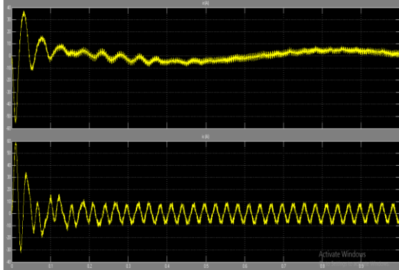
Fig 6: Waveforms Of Rotor And Stator Current Of Three Phase Induction Motor for m_a=0.7
