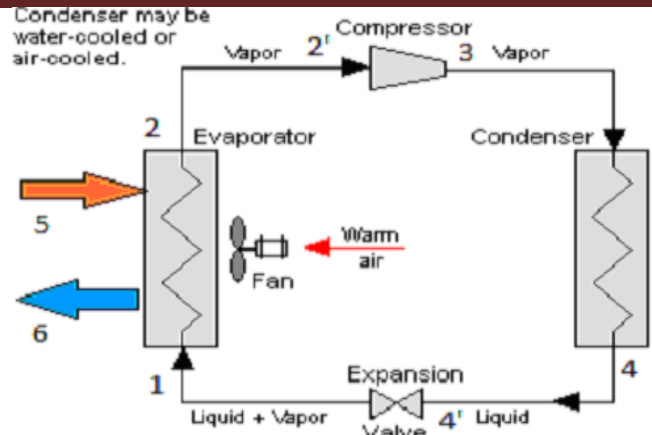
Fig. 1 Vapor Compression Refrigeration System
