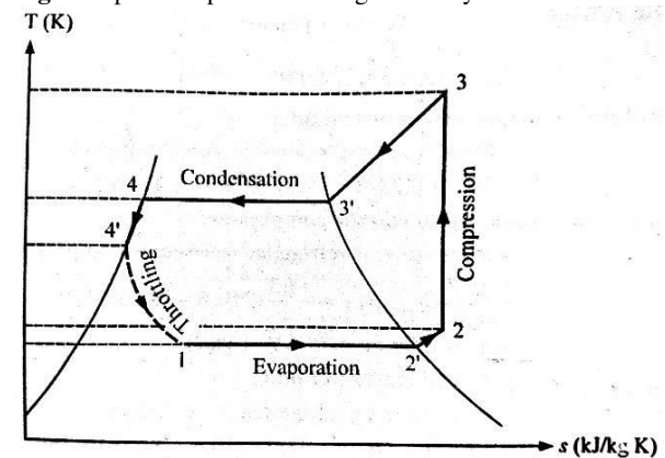
Fig. 2 T-s Diagram of VCERS
