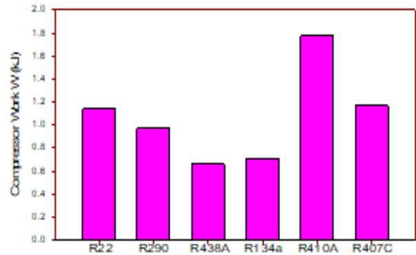
Fig. 3 Comparison of Compressor Work
