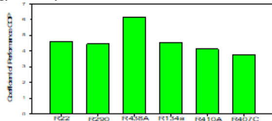
Fig. 5 Comparison of Coefficient of Performance
