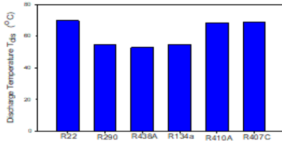
Fig. 6 Comparison of Discharge Temperature stability.
